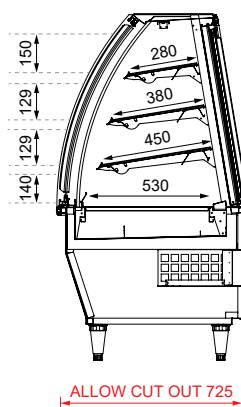
SECTION VIEW
