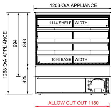
FRONT ELEVATION
