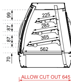
SECTION VIEW
