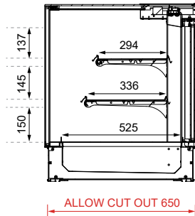
SECTION VIEW
